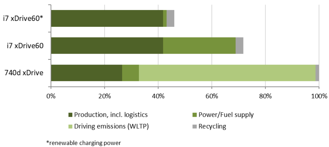
Fig. 2: Distribution of global warming potential over life cycle of BMW i7 xDrive60 in relation to the conventional 740d xDrive
