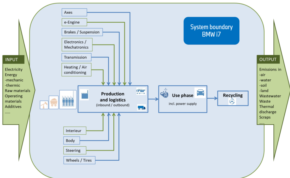
Fig. 1: Flowchart input / output data of the BMW i7
