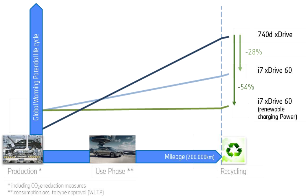
Fig. 3: Classification of the BMW i7 xDrive60 in relation to a conventional vehicle concept (740d xDrive)
